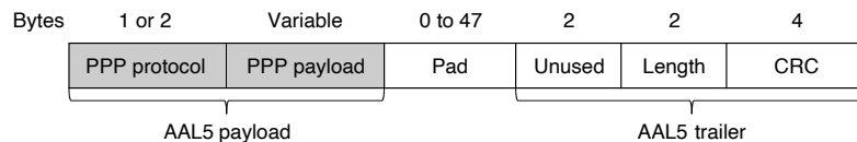
Figure 3-27. AAL5 frame carrying PPP data.
